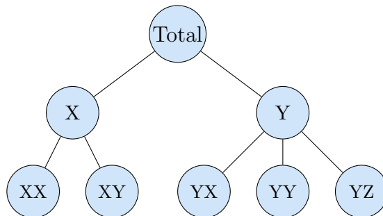
Figure 2: An example hierarchy of time series.
